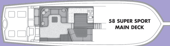
58 SUPER SPORT MAIN DECK SPIRAL STAIRCASE (OPTIONAL)
